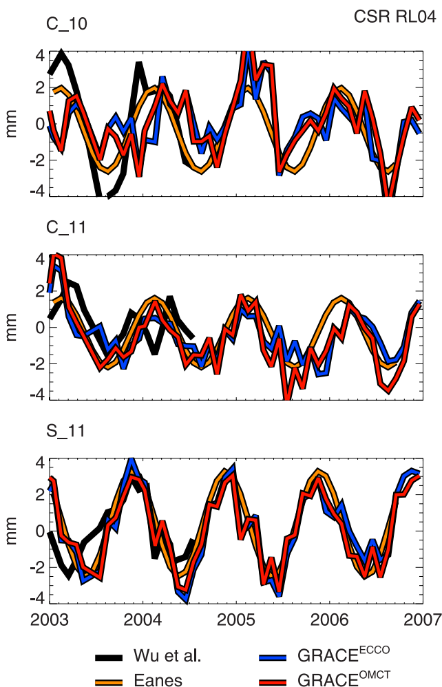
Figure 3. Time series of full geocenter estimates computed using GRACE Stokes coefficients and degree one ocean model results. Blue and red lines are derived from equation (12) using ECCO and OMCT ocean models, respectively, after adding a eustatic correction to each model. Black line represents values estimated by Wu et al. [2006] , and orange line represents mean seasonal estimate from Eanes [2000] . (top) Z . (middle) X . (bottom) Y . The y axis is in millimeters. The x axis is time in years.
