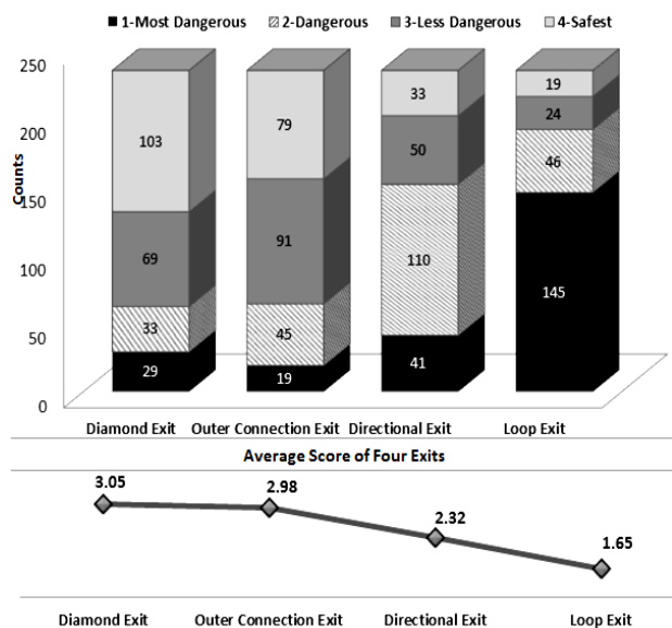
Figure 6. Counts of each score and average scores by four exit types based on web-survey data.
