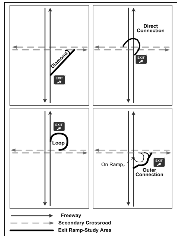
Figure 1. Four typical exit ramp types.
