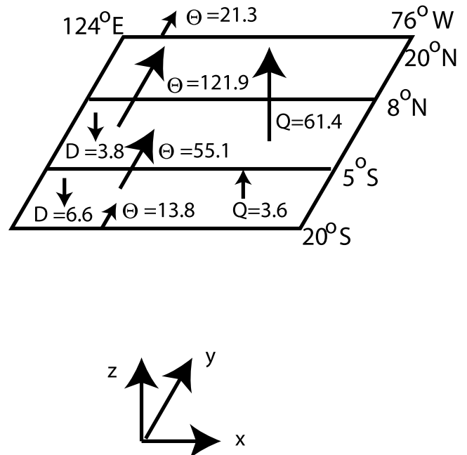
Figure 9. Schematic of volume tendency effects for the 20^{\circ}\text{S} – 20^{\circ}\text{N} box, subdivided at 5^{\circ}\text{S} and 8^{\circ}\text{N} . The region is shown as an inclined plane. Only terms which are equivalent to at least 3% of the 20^{\circ}\text{S} – 20^{\circ}\text{N} volume change are included here. This includes the heat fluxes at the sea surface, Q ; heat fluxes across the meridional faces, \theta ; and mismatches in the temperature equation, D . The number next to the arrow indicates the relative importance of each term.
