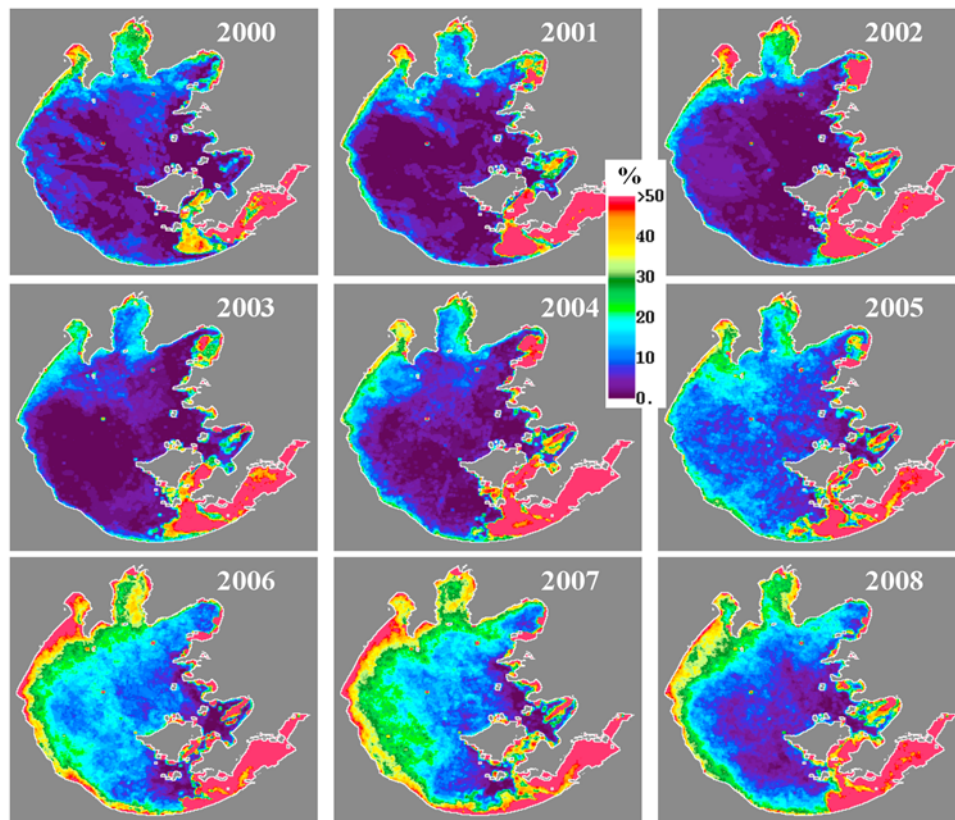
Figure 6. Percentage of MODIS measurements when cyanobacteria blooms (FAI > -0.004) were found from MODIS FAI imagery.
