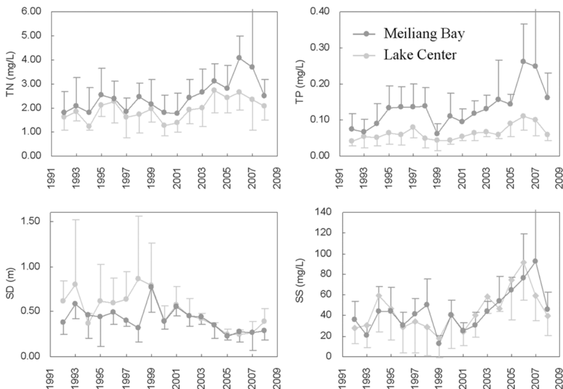
Figure 11. Total nitrogen (TN), total phosphorus (TP), transparency (Secchi disk depth (SD)), and suspended solids (SS) in the lake center and Meiliang Bay during summer 1991–2008. Adapted from Zhu [2008], but with more recent data for 2007 and 2008.
