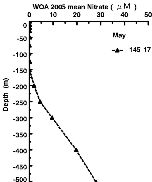
Figure 8. Climatological nitrate profile for the month of May in the WNOPSG. Profile location is annotated by a triangle in Figure 1b (data source: NOAA World Ocean Atlas 2005 [Garcia et al. , 2006]).
