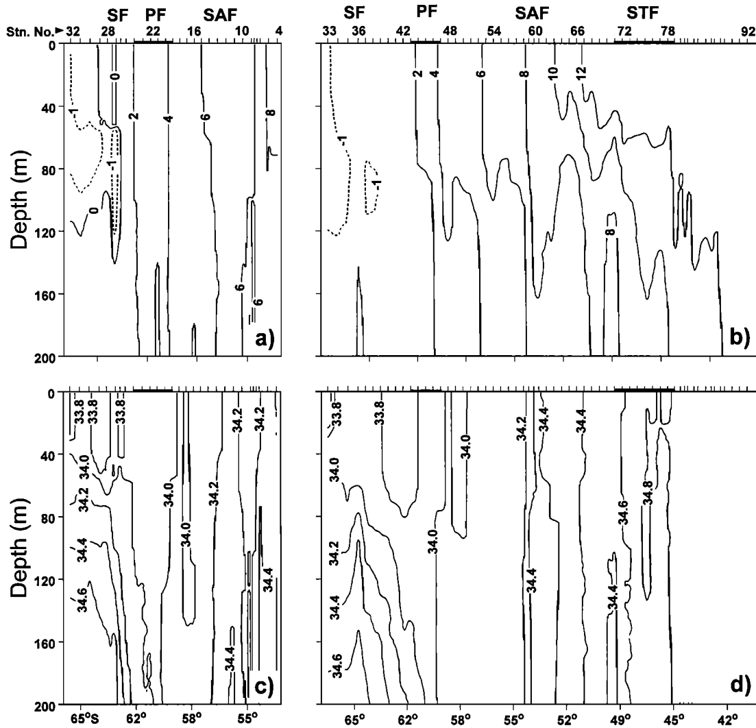
Figure 2. The distribution of (a and b) potential temperature (°C) and (c and d) salinity. Data are continuous measurements from conductivity-temperature-depth (CTD) profiles. Here and in Figures 3–9 the locations of the Southern Front (SF), the Polar Front (PF), the Subantarctic Front (SAF), and the Subtropical Front (STF) and station numbers are indicated above the top panels; the dark bar under PF and STF indicates the northern and southern branches of these fronts; latitude (°S) is shown below the bottom panels. Left and right panels are hydrographic sections P14S and P15S, respectively.
