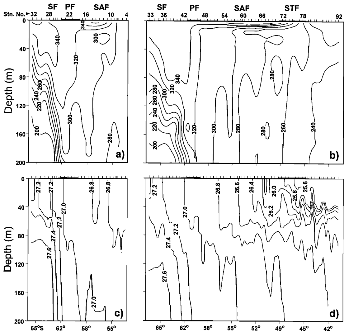
Figure 3. The distribution of (a and b) oxygen ( \mu\text{mol kg}^{-1} ) and (c and d) density (expressed as \sigma_t ). Left and right panels are hydrographic sections P14S and P15S, respectively.
