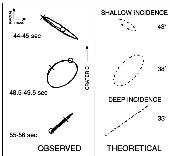
Figure 4. Observed and theoretical particle motions in the horizontal plane. The left column shows a 12 s sequence (0.5-3 Hz bandpass) taken from the second tremor episode ("B") in figure 3. An "x" marks the beginning and an "o" the end of each one-second trace. The particle motion azimuth abruptly rotates clockwise 105^\circ . The right column shows theoretical particle motions on a horizontal free surface due to a shear wave (polarization angle \epsilon = 20^\circ , Poisson's ratio = 0.25) incident at three angles (measured from the vertical). The observed tremor particle motions may be explained by an apparent steepening of the incidence angle.
