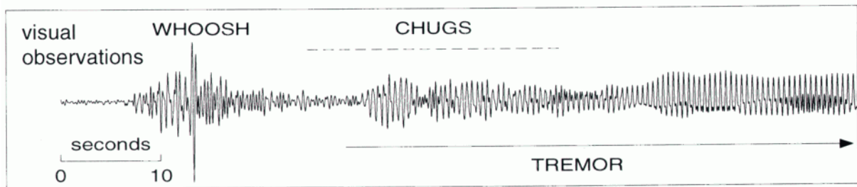
Figure 2. An example seismogram (radial component) of a small eruption (whoosh) followed by rhythmic degassing (chugs). Visual and audio observations show this eruption ejecting ash to ~500 m above the crater and the following chugs were audible at 2.8 km for ~25 s. Harmonic tremor begins during the chugs and continues for several minutes.
