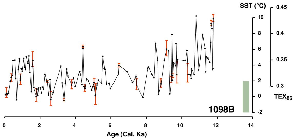
Figure 1. TEX 86 SST record from ODP Site 1098 (Palmer Deep) on the western Antarctic Peninsula continental margin. The 1s temperature error bars are shown in red for replicated data; 20% of the data has been replicated (SDp: ±0.5°C). The green bar represents the range of average Austral Spring-Fall sea surface temperatures observed in Palmer Deep.
