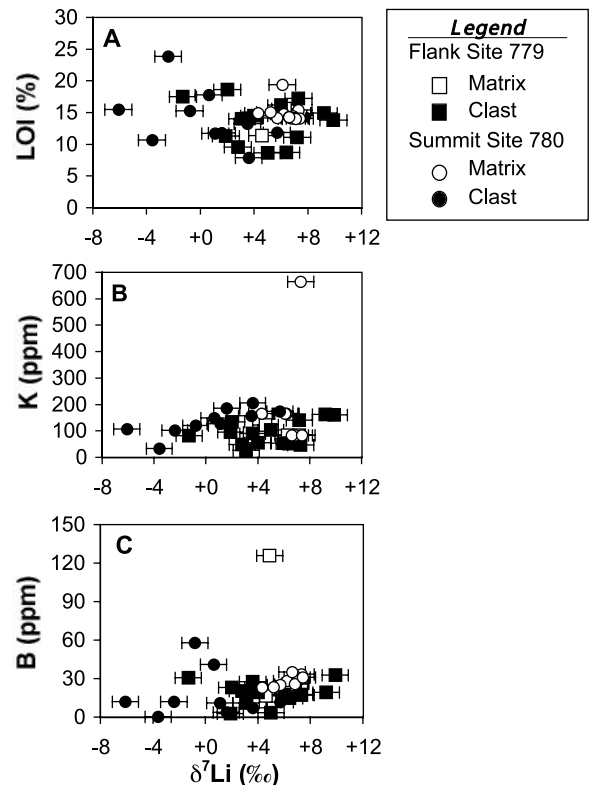
Figure 5. Plots of (a) \delta^7\text{Li} versus LOI; (b) \delta^7\text{Li} versus K concentrations; and (c) \delta^7\text{Li} versus B concentrations for Leg 125 serpentinites. Additional data are from Benton et al. [2001] and Mattie and Ryan [1994].
