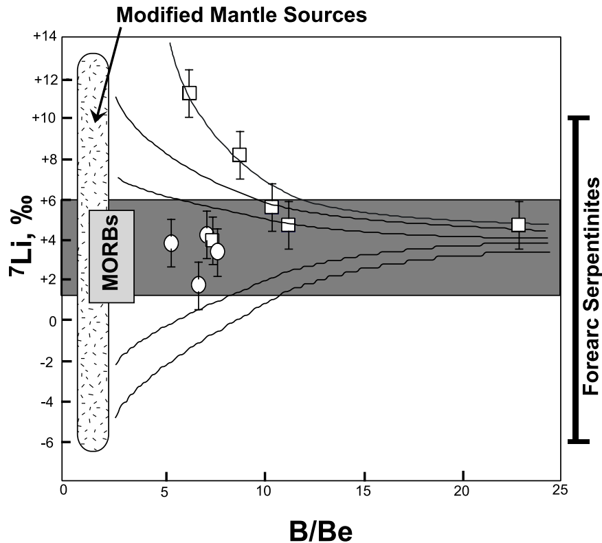
Figure 9. Plot of \delta^7\text{Li} versus B/Be for arc lavas. The darkly shaded field across the diagram represents the combined \delta^7\text{Li} arc data sets of Chan et al. [1999, 2001] and Tomascaak et al. [2002], which constitute most of the available data on “normal” arcs, and overlaps entirely with the range for MORBs (labeled [ Tomascaak and Langmuir , 1999]). The symbols represent Old Group (squares) and Young Group (circles) arc lavas from Panama [ Tomascaak et al. , 2000]. The range of \delta^7\text{Li} for the Mariana forearc serpentinites is shown by the large bracket to the right of the plot. The stippled vertical field represents the range of possible \delta^7\text{Li} signatures developed in the mantle wedge over time via slab fluid exchange, and the curves represent hypothetical mixing arrays between these mantle reservoirs and slab fluid, which has high B/Be, and (in most arcs) relatively MORB-like \delta^7\text{Li} .
