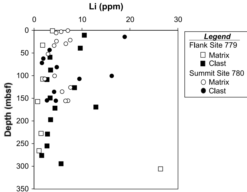
Figure 2. Plot of Li concentrations for Leg 125 serpentinites versus depth in core. Matrix and clast samples from each drill site are as noted on the diagram; matrix samples are open symbols, and clast samples are solid symbols.
