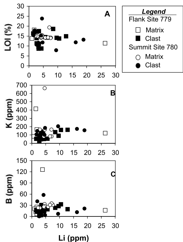
Figure 3. Plots of (a) Li concentrations versus LOI; (b) Li versus K concentrations; and (c) Li versus B concentrations for Leg 125 serpentinites. Additional data are from Benton et al. [2001] and Mattie and Ryan [1994].
