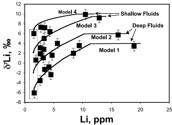
Figure 8. Plot of \delta^7\text{Li} versus Li concentrations for the Leg 125 serpentinized clast samples. The four trend lines represent possible serpentine compositions developed during progressive fluid/rock serpentinization reactions with fluids derived from deeper (Models 1 and 2) and shallower (Models 3 and 4) portions of the slab. Serpentine compositions were calculated incrementally using the equilibrium fluid/rock exchange equation [Nabelek, 1987, equation (3)]: C_r^f = (C_r^i + NC_w^i)/(D_s^i N + 1) for Li concentrations and R_r^f = [(R_r^i + 1000) + N(R_w^i + 1000)]/(\alpha_s^i N + 1) - 1000 for \delta^7\text{Li} values. C_r represents concentrations in the rock, C_w is concentrations in the fluids, R_r is the \delta^7\text{Li} of the rock, and R_w is the \delta^7\text{Li} of the fluid; D_s^i is the fluid/solid distribution coefficient for Li (set at 3.5 [Scambelluri et al., 2004]), and \alpha_s^i is the Li isotope fractionation factor (set at 1.015, assuming higher temperatures than encountered during exchanges on the seafloor [e.g., Chan et al., 1992]). Initial fluid Li concentrations and isotope ratios were estimated on the basis of the values necessary to produce the high-Li, high- \delta^7\text{Li} samples along each trend. Fluid/rock ratios begin at 1.5 for the deep fluid trends and at 2.3 for the shallow fluid trends. The Li concentration of the mantle is set at 1.5 ppm [Ryan and Langmuir, 1987; Seitz and Woodland, 2000], while mantle \delta^7\text{Li} values were selected to best approximate the trends of our data. Fluid/rock ratios were reduced with each increment calculated to reflect the incorporation of fluids into forming serpentines; increment sizes were kept small so as to approximate continuous fluid/rock exchange during serpentine formation. The large range of \delta^7\text{Li} in both the high-Li and low-Li serpentinite clasts necessitates multiple fluid/rock exchange trajectories with fluids of different initial \delta^7\text{Li} and lithium concentrations, and a mantle that is already zoned in terms of Li isotopic composition.
