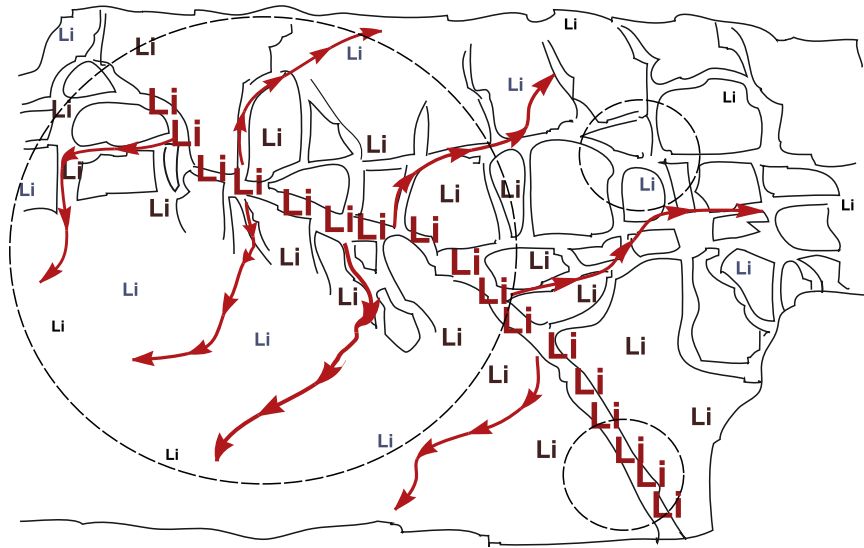
Figure 7. Sketch of a veined Mariana forearc serpentinite showing a likely pattern of Li distribution due to exchanges with vein fluids. Slab-derived fluids inject Li (red lettering), which is largely deposited in serpentinite near the vein. Percolation of fluid outward from the vein forms serpentinite with progressively lower Li content (brown to blue to black lettering). Subsequent fluid injections will overprint this pattern, producing serpentinites with highly variable Li contents. Lithium isotope ratios in the forming serpentinite will vary on the basis of depths of fluid origin and the composition of the mantle, though high-Li samples will have higher \delta^7\text{Li} (see also Figure 8). Dashed circles overlain on the sketch represent the kind of sampling of this modified mantle that could occur during melting: small F melts will preferentially sample the most hydrated portions of the subarc mantle, but these portions may have either high or low \delta^7\text{Li} . Melting at larger values of F will average greater volumes of mantle, producing lavas with intermediate (and relatively uniform) \delta^7\text{Li} .
