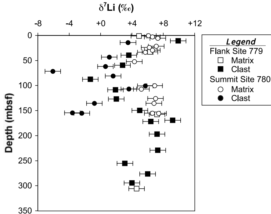
Figure 4. Plot of \delta^7\text{Li} for Leg 125 serpentinites versus depth in core.
