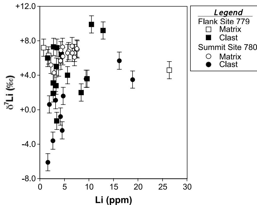
Figure 6. Plot of \delta^7\text{Li} versus Li concentrations for Leg 125 serpentinites.
