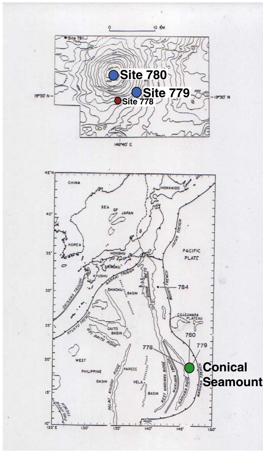
Figure 1. Map of the Mariana forearc region, with close-up of the Conical Seamount showing the location of Sites 779 and 780. From Fryer [1992].
