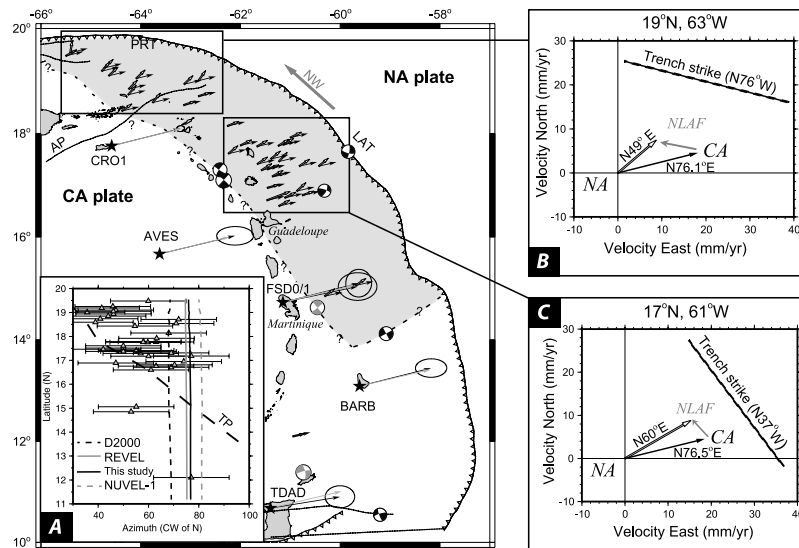
Figure 2. Slip partitioning and the possible NLA block. Maps shows deviation of slip vectors (white arrows) from predictions (black arrows) of our 9-site CA-NA Euler vector. Black (0–20 km) and gray (20–40 km) strike-slip focal mechanisms are from the Harvard CMT catalog. (a) Azimuths of shallow thrust slip vectors (triangles) and predictions of various Euler vectors. TP = trench normal azimuth. D2000 from DeMets et al. [2000]. (b) and (c) Average SV azimuths (white vector) from two regions show misfit to predicted azimuth (black vector) at those locations, suggesting the presence of a block moving WNW with respect to CA.
