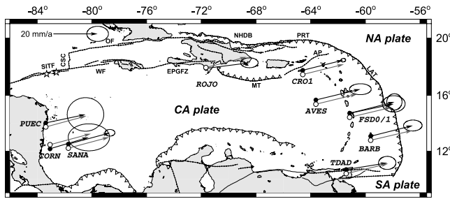
Figure 1. Regional tectonic map. Black circles and vectors with 2\sigma error ellipse are velocities of sites in a NA reference frame. Open circles with gray vectors (offset for clarity) are velocities predicted by our 9-site GPS-only CA-NA Euler vector. ROJO, previously considered as a stable CA site, was not used in the inversions. AP-Anegada Passage, CSC-Cayman Spreading Center, EPGFZ-Enriquillo-Plantain Garden Fault Zone, LAT-Lesser Antilles Trench, MT-Muertos Trough, NHF-Northern Hispaniola Fault, OF-Oriente Fault, PRT-Puerto Rico Trench, SITF-Swan Island Transform Fault.
