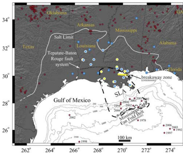
Figure 1. Map of GPS sites in Louisiana superimposed on a shaded relief map: continuous sites (cyan), episodic sites (yellow). Sites with white border are plotted in Figure 2 (see Table S1 of the auxiliary material). White line labeled “Salt Limit” shows northern limit of sub-surface salt layers. Boundary of southeast Louisiana allochthon (SLA) shown as heavy black dashed line; based largely on the south vergent, coupled extensional-contractional system of Peel et al. [1995]. Actual detached area may extend into Texas. Mississippi Fan Fold Belt is a zone of folded Holocene sediments undergoing contraction synchronous with south translation of SLA and extension in breakaway zone. Breakaway zone marked by Michoud fault (yellow line), but is likely more complex and includes more northerly faults belonging to the Tepatate-Baton Rouge system. This system marks the approximate northern edge of lithosphere thinned during Jurassic rifting of the Gulf of Mexico [Worrall and Snelson, 1989]. Earthquakes 1978–2006 (red stars), source is U.S. Geological Survey, http://neic.usgs.gov/neis/epic/epic.html . Bathymetric contours are in meters.
