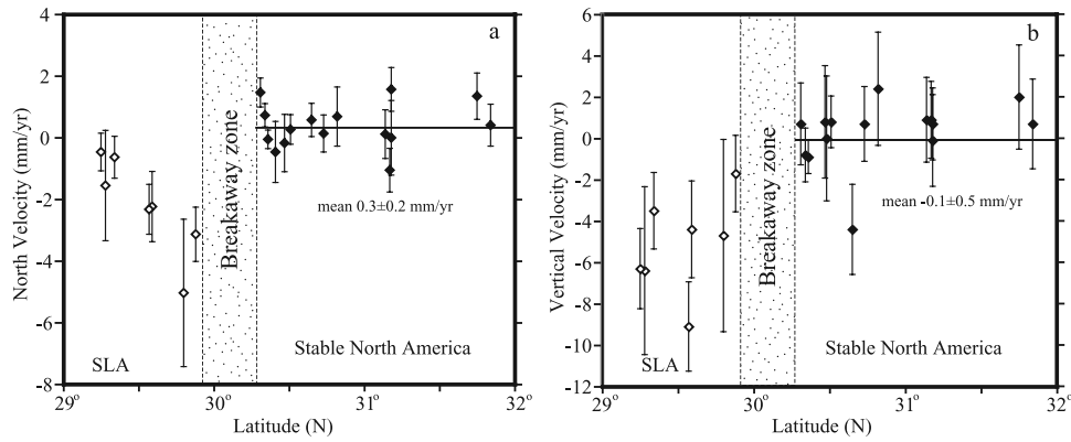
Figure 2. (a) North and (b) vertical components of GPS site velocities for sites with white border in Figure 1, plotted as a function of latitude. North component is relative to stable North America [Sella et al. , 2006]. Vertical stippled zone is approximate location of breakaway zone. Open diamonds are sites located south of fault; solid diamonds are sites north of fault. Error bars for individual data are 1 standard deviation. Horizontal line depicts the mean of GPS data for areas north of breakaway zone.
