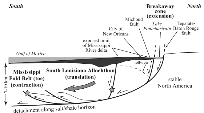
Figure 3. Cartoon depicting the regional scale, extensional-contractional complex comprising the south Louisiana allochthon (adapted from Peel et al. [1995]). The system is driven by loading due to late Quaternary deposition of the Mississippi River delta (black shaded area) and eustatic sea level rise. Southward translation of the south Louisiana allochthon with respect to stable North American plate is accompanied up dip by extension in the breakaway zone by normal faulting, and down dip by contraction in the Mississippi fold belt. Non-uniform horizontal motions implied by GPS observations and earthquakes suggest that the allochthon is only partially intact. Tectonic subsidence along faults of the breakaway zone occurs because of downward motion of the hanging wall, and local reverse drag. Reverse drag is the consequence of translation along a curved fault plane and results in a rollover antiform. Local subsidence is due to the integrated effects of regional isostasy, faulting, sediment compaction, dewatering, and fluid withdrawal. Small arrows show relative fault motions.
