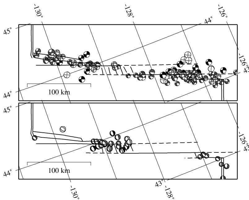
Figure 10. Fault plane solution map (lower hemisphere projection, size proportional to M_w ). (top) Plot of 115 strike-slip, (bottom) plot of 31 normal faulting events. Black indicates relocated RMT solutions (latitude and longitude uncertainty \leq 12 km); dark gray indicates RMTs on SOSUS location; medium gray indicates RMTs located with regional P and S arrival time data for events without SOSUS location; light gray indicates relocated CMT solutions. Events are listed in Tables 2 and 3.
