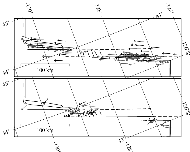
Figure 11. (top) Map of slip vector azimuths of the 115 strike slip earthquakes. (bottom) Map of T axis orientations of the 31 normal faulting events. Gray scheme is as in Figure 10.
