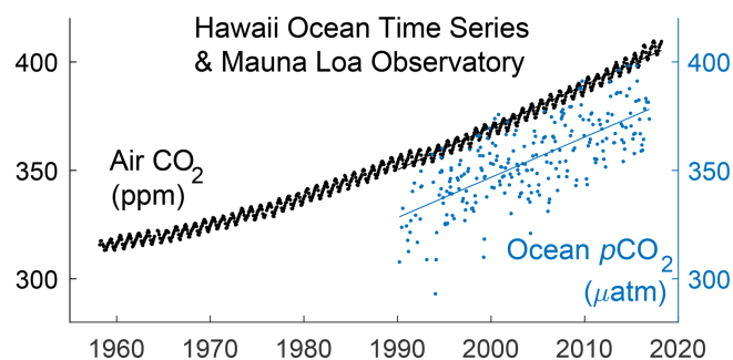
Figure 6. Atmospheric CO 2 (black dots) measured at the Mauna Loa Observatory in Hawaii beginning in 1958 and surface ocean pCO 2 data (blue dots) from the Hawaii Ocean Time Series (HOT) station (see Fig. 3 for site location). Black and blue lines indicate linear trends after 1990. Atmospheric CO 2 increased by 1.86 \pm 0.11 \text{ ppm yr}^{-1} . Surface ocean pCO 2 increased by 1.95 \pm 0.017 \mu\text{atm yr}^{-1} . pCO 2 is calculated using CO2SYS, with Mehrbach refit coefficients for the dissociation constants of H 2 CO 3 and HCO 3 - , and Dickson's dissociation constant for HSO 4 - . Data sources: Mauna Loa ( http://www.esrl.noaa.gov/gmd/ccgg/trends/data.html , last access: 1 May 2018); HOT ( http://hahana.soest.hawaii.edu/hot/hot-dogs/interface.html , last access: 1 May 2018).
