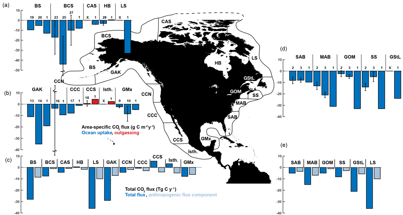
Figure 4. North American continent with EEZ decomposition (indicated by black outlines). Selected area-specific regional CO 2 flux estimates from Fig. 2 are shown in comparison to the global model estimates (referred to as 1) in (a, b, d) (see Fig. 2 for reference key). “X” indicates that no regional estimate is available. Total CO 2 flux estimates from the global model and the anthropogenic components are shown in (c, e). Subregion abbreviations are MAB – Mid-Atlantic Bight, GOM – Gulf of Maine, SS – Scotian Shelf, GSStL – Gulf of St. Lawrence and Grand Banks, LS – Labrador shelf, HB – Hudson Bay, CAS – Canadian Arctic shelf, BCS – Beaufort and Chukchi seas, BS – Bering Sea, GAK – Gulf of Alaska, NCCS – northern California Current System, CCCS – central California Current System, SCCS – southern California Current System, Isthmus – American isthmus, GMx – Gulf of Mexico and Yucatán Peninsula, SAB – South Atlantic Bight.
