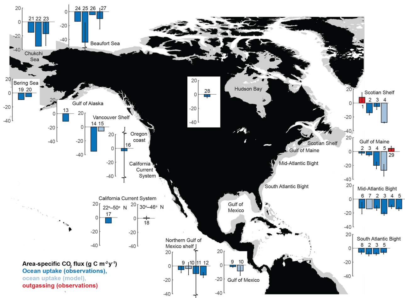
Figure 2. Observation- and model-based estimates of regional net air–sea \text{CO}_2 flux in \text{g C m}^{-2} \text{yr}^{-1} . Positive fluxes (red bars) indicate a flux to the atmosphere. Observation-based estimates are shown in red and dark blue. Model-based estimates are in light blue. Broken error bars are used where errors bars reach outside the range of the y axis. References: (1) Shadwick et al. (2010), (2) Signorini et al. (2013) using Ho et al. (2011) gas transfer parameterization, (3) satellite-based estimate from 2, (4) Fennel and Wilkin (2009), (5) Cahill et al. (2016), (6) DeGrandpre et al. (2002), (7) Fennel et al. (2008), (8) Jiang et al. (2008), (9) Robbins et al. (2014), (10) Z. Xue et al. (2016), (11) Huang et al. (2015), (12) Lohrenz et al. (2018), (13) Evans and Mathis (2013), (14) Evans et al. (2012), (15) Ianson and Allen (2002), (16) Evans et al. (2011), (17) Hales et al. (2012), (18) Turi et al. (2014), (19) Cross et al. (2014b), (20) Takahashi et al. (2009), (21) Evans et al. (2015b), (22) Gao et al. (2012), (23) Yasunaka et al. (2016), (24) Shadwick et al. (2011), (25) Else et al. (2013), (26) Evans et al. (2015b), (27) Mucci et al. (2010), (28) Else et al. (2008), (29) Vandemark et al. (2011). The flux estimates are also reported in Table S1 in the Supplement.
