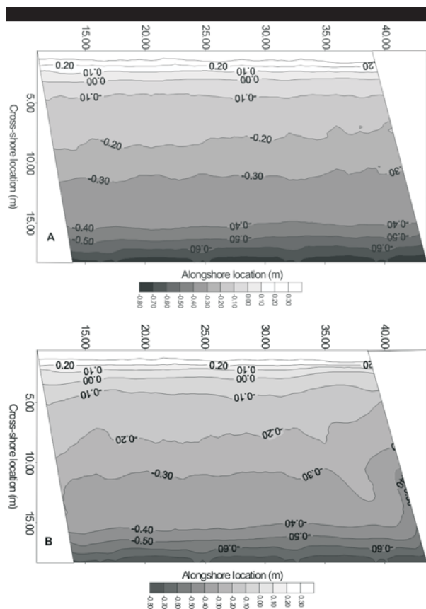
Figure 2. Uniformity of the test beach. A: directly after restoration; B: directly before restoration.
