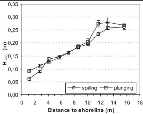
Figure 4. Alongshore uniformity of wave height.
