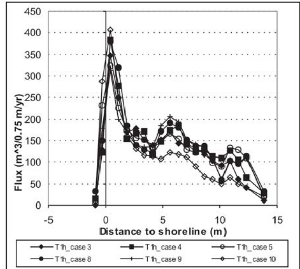
Figure 6. Repeatability of cross-shore distribution of longshore sand transport.
