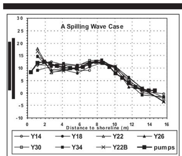
Figure 3. Pumps settings and the longshore-current uniformity. Numbers in the legend represent different alongshore locations.
