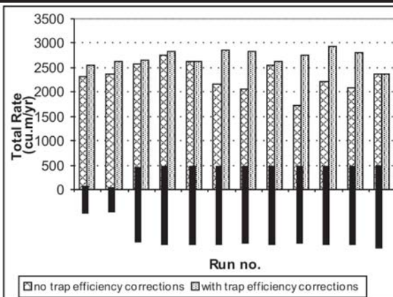
Figure 5. Trapping efficiency at the downdrift bottom traps.
