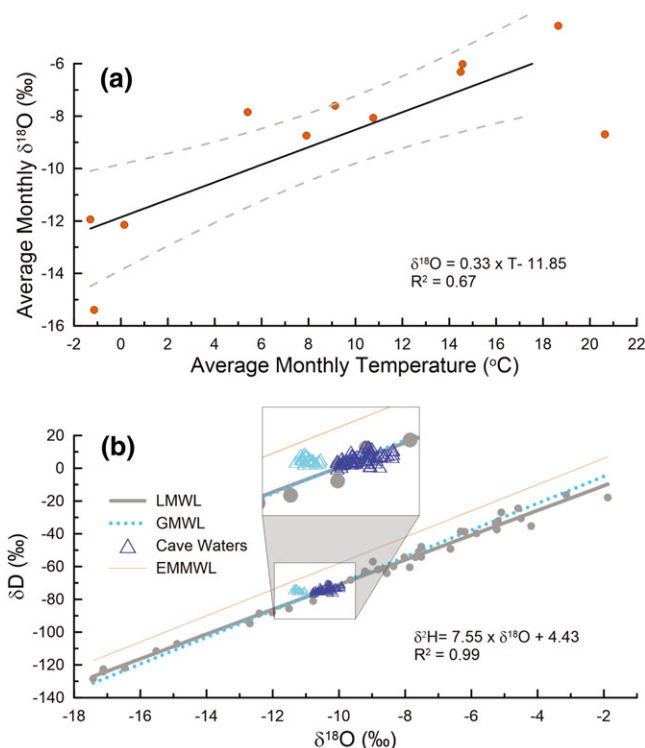
FIGURE 2 (a) Average monthly air temperature plotted against monthly rainwater \delta^{18}\text{O} for the period 2010–2011 at Urşilor Cave. Dashed grey lines indicate the confidence interval of the regression, (b) the Local Meteoric Water Line (LMWL) at Urşilor Cave compared with the Global Meteoric Water Line and the Eastern Mediterranean Meteoric Water Line. Grey circles indicate the stable isotope composition of rainwater and the dark blue triangles show the stable isotope values of dripwaters. Cyan triangles indicate the isotopic values of dripwaters affected by freezing conditions
