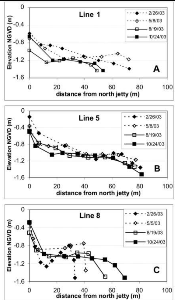
Figure 6. Patterns of sediment accumulation and erosion over the northern shoal. Locations of the lines are plotted in Figure 2.
