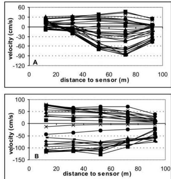
Figure 4. Cross-channel distribution of tidal flow, measured over a spring tidal cycle. A: near the Gulf entrance; B: near the bent.
