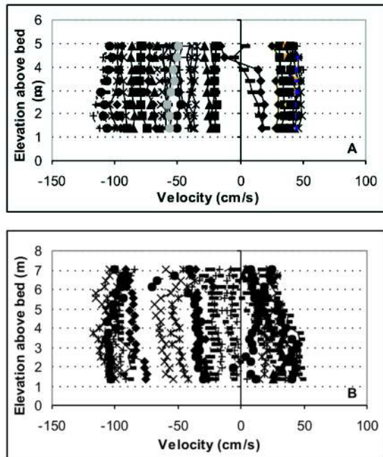
Figure 3. Profiles of tidal current measured in the main channel over a spring tidal cycle. A: current velocities measured in January 2001; B: currents measured in November 2002.
