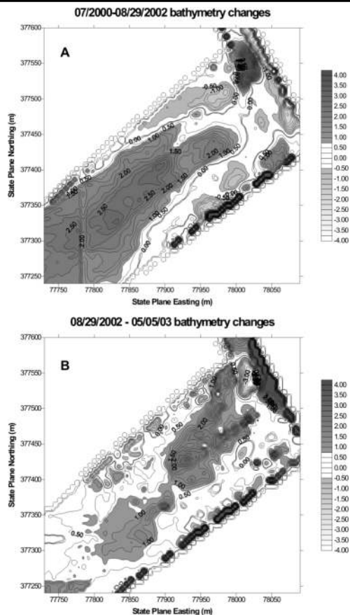
Figure 5. Patterns of sedimentation and erosion. White areas represent areas with less than 0.5 m sedimentation or erosion. Depth is referred to mean low tide. A: bathymetry changes between 07/2000 and 08/2002; B: bathymetry changes between 08/2002 and 05/2003.
