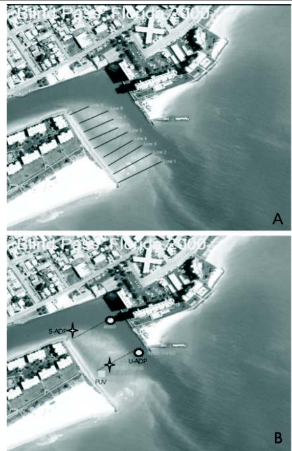
Figure 2. Locations of the nine level-and-transit survey lines (A) and current meters (B).
